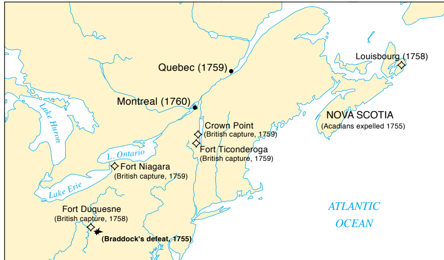
Events of 1755–1760
